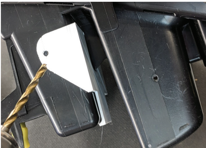
Align the template on the housing as shown. Drill hole here and on other side
